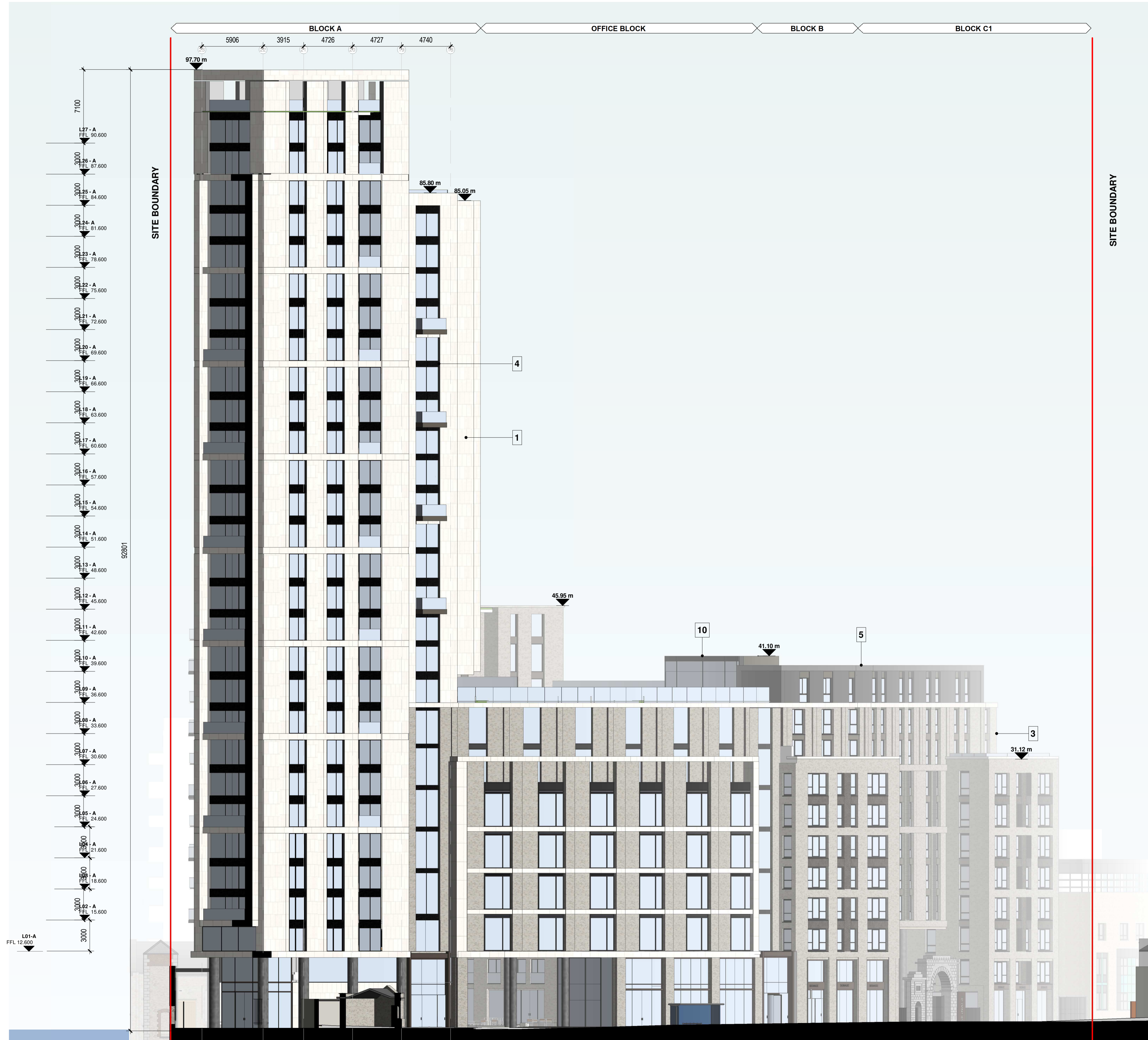
Proposed North East Elevation 1 : 200
